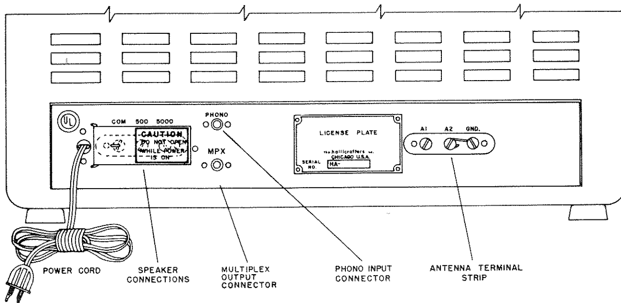
Figure 2. Rear View
