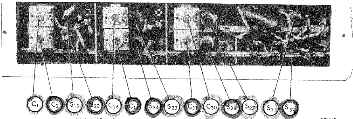
Fig. 10 Alignment adjustments, left side view
