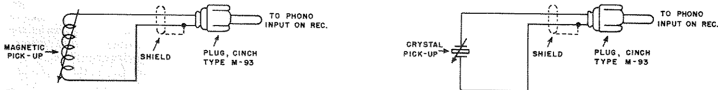
Fig. 4. Wiring diagram, record player connection.
