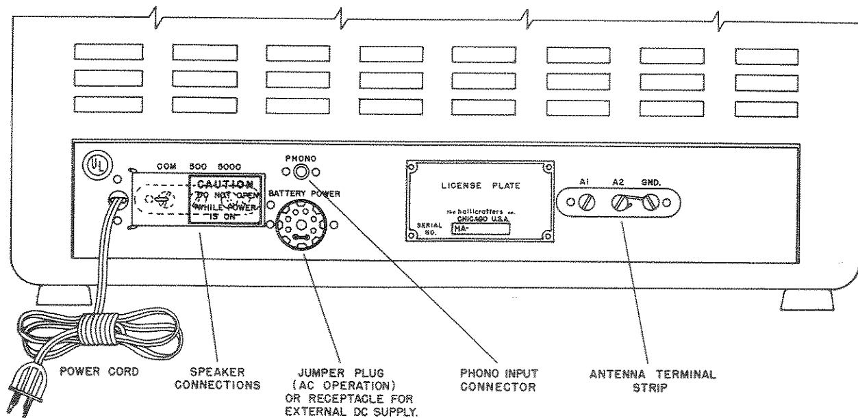
Fig. 3. Rear view.
