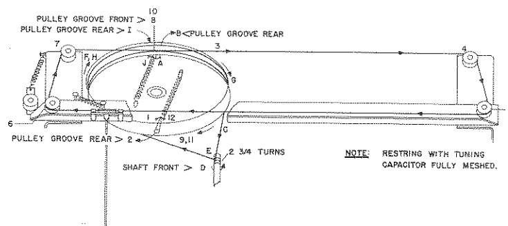
Fig. 7. Dial cable stringing procedure
