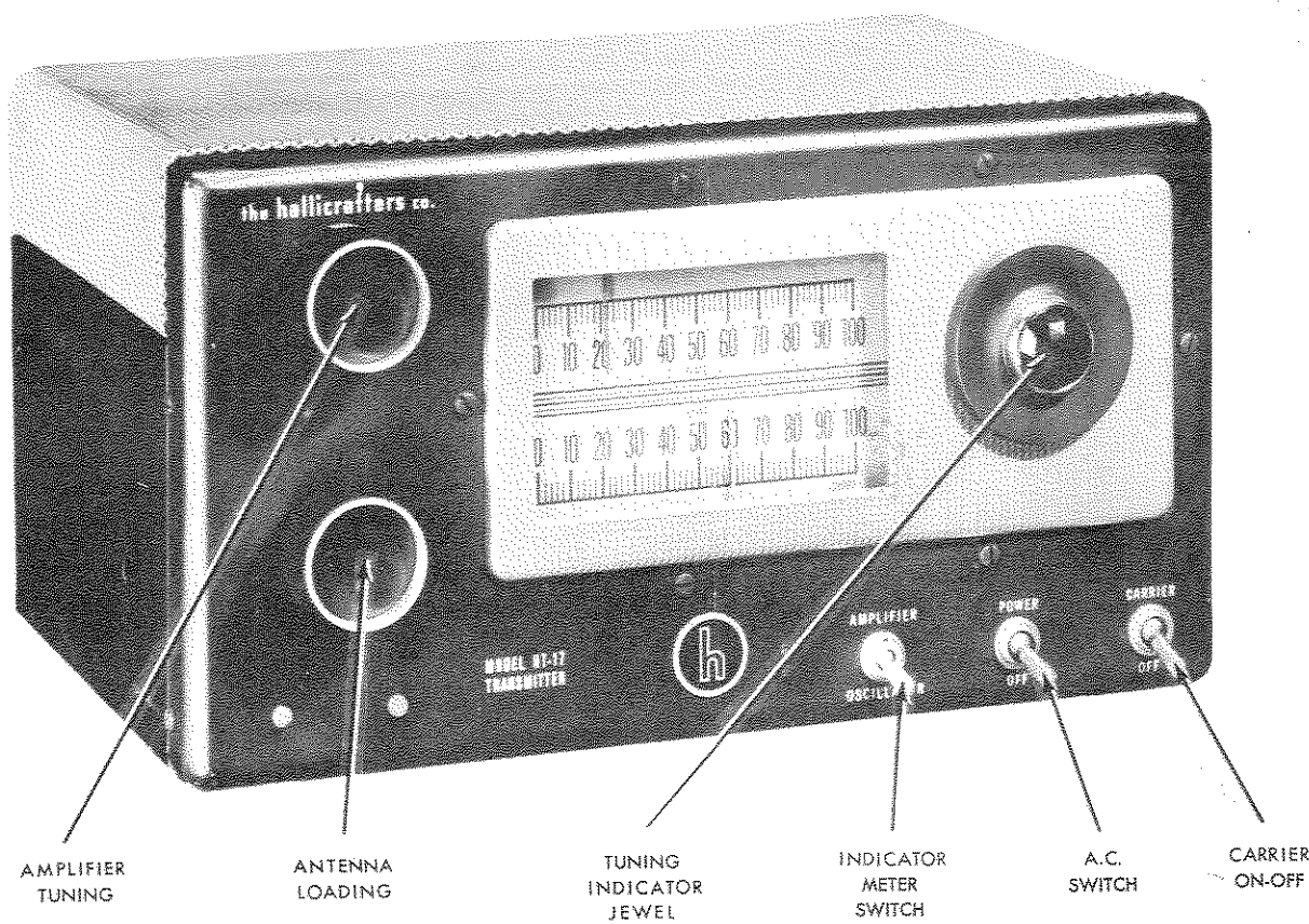
Figure 1. Front View, showing location of controls.
