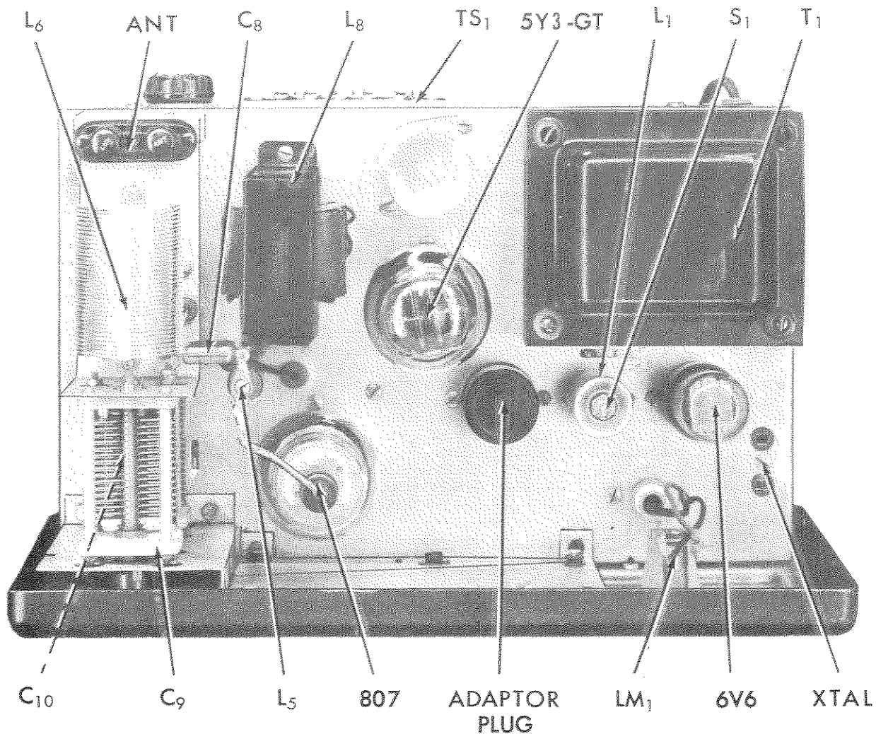
Figure 3. Top View of Chassis.
