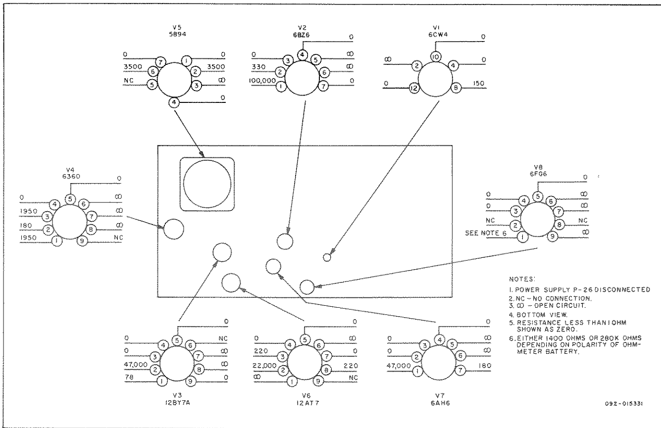
Figure 8. Resistance Chart.
