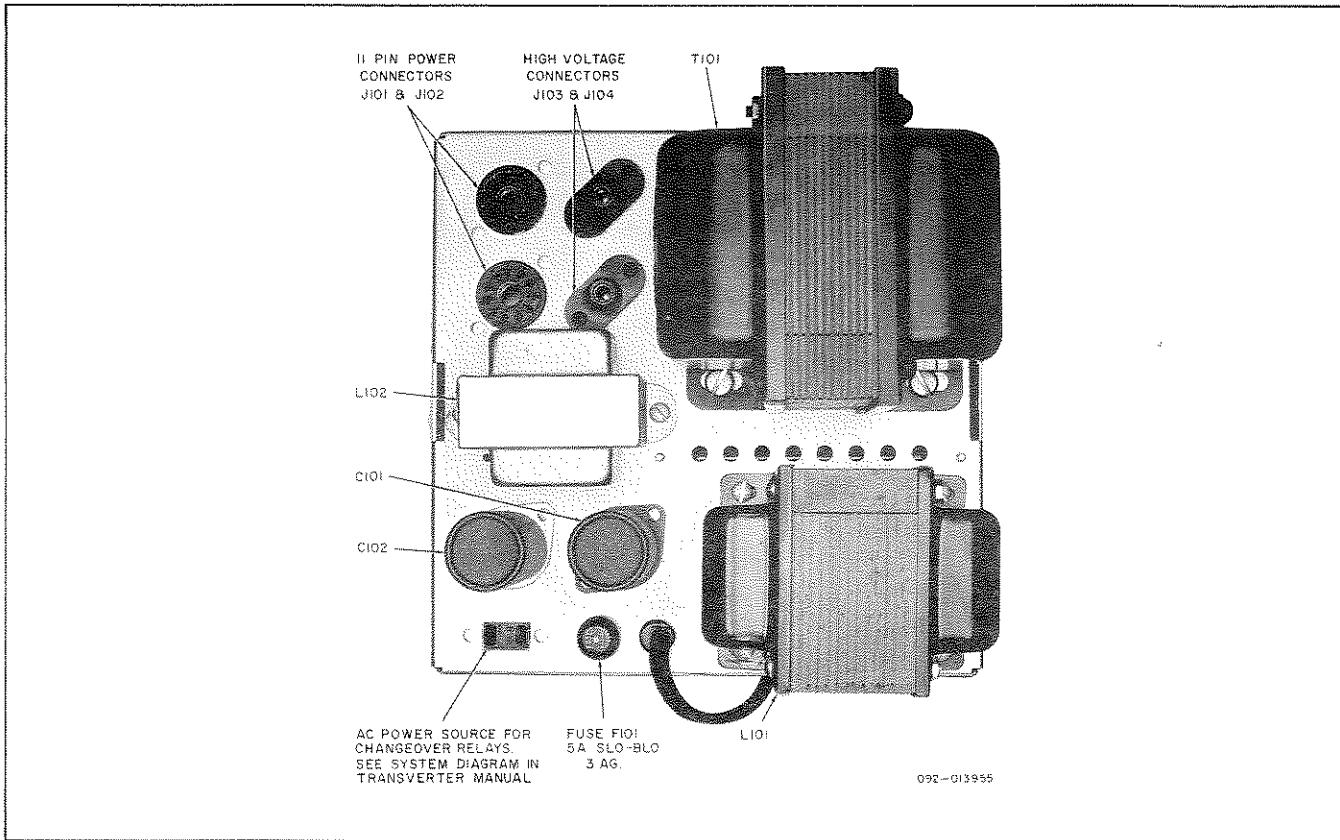
Figure 13. Top View of P-26 Power Supply.
