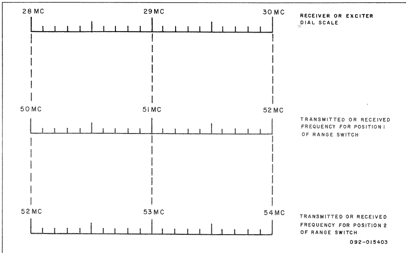
Figure 5. Frequency Conversion (Dial Scale Interpolation).
