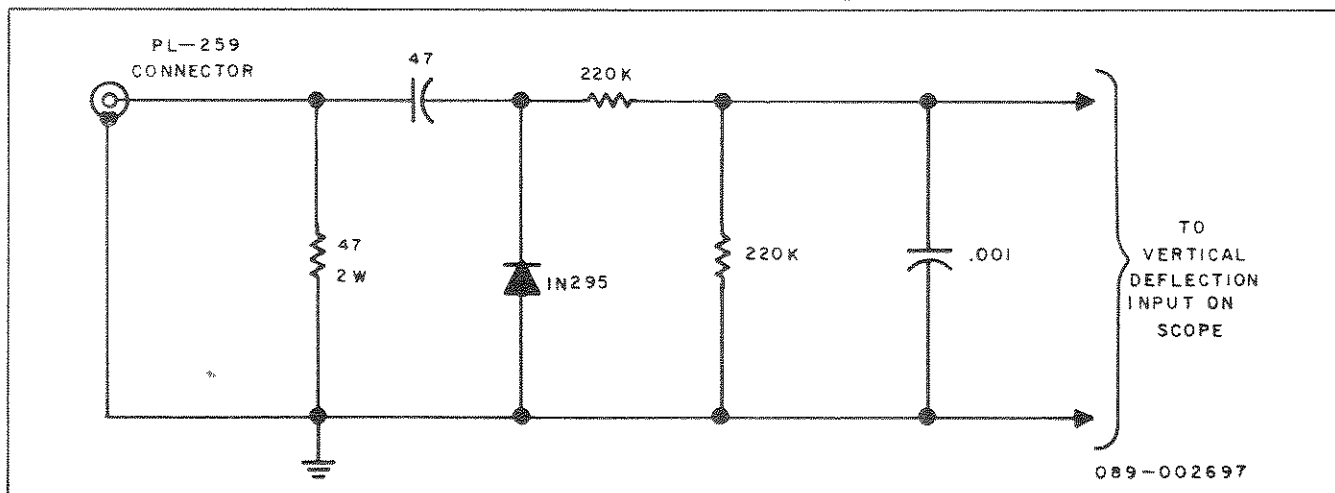
Figure 11. Diode Detector.
