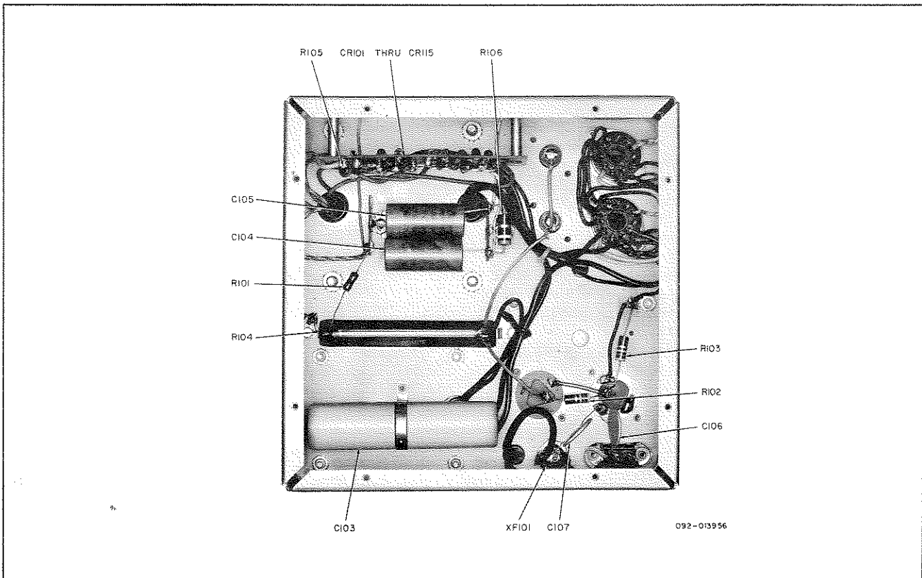
Figure 14. Bottom View of P-26 Power Supply.
