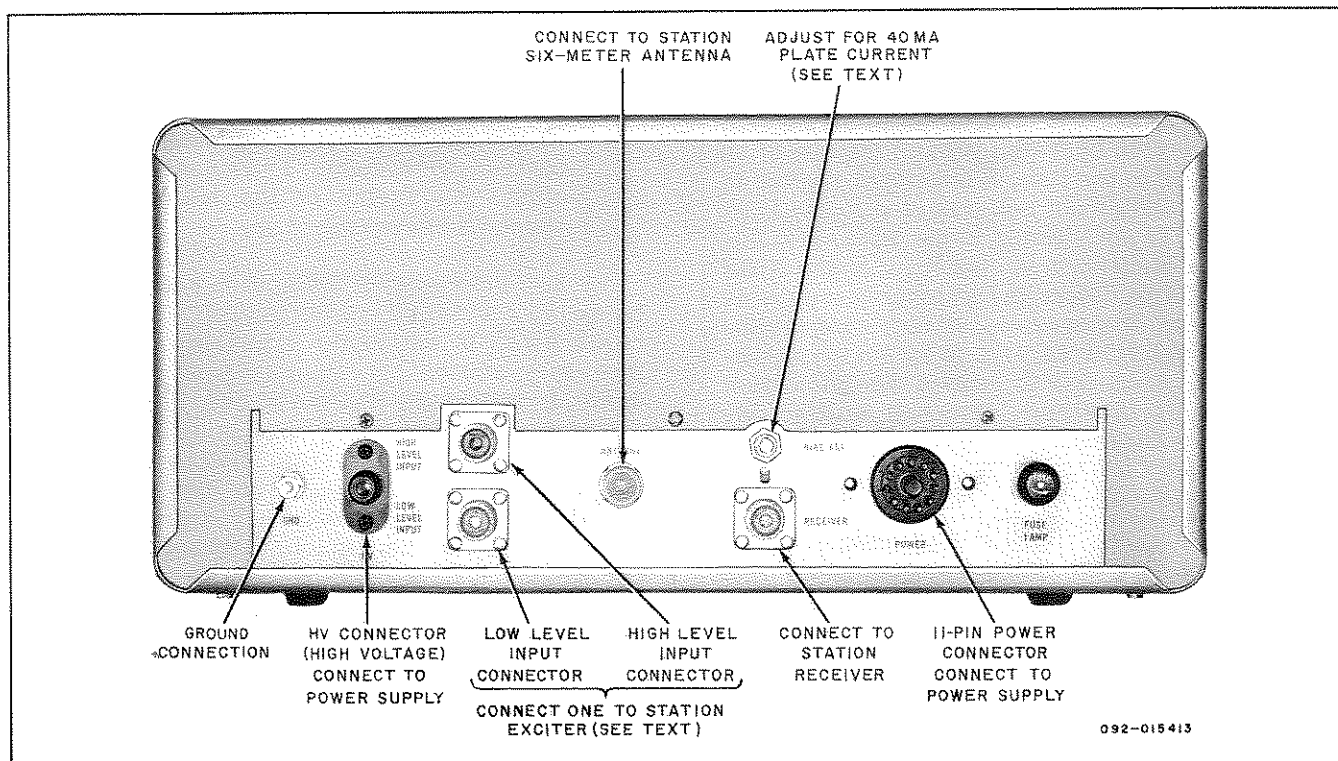
Figure 2. Rear View of Transverter, Showing Connectors.
