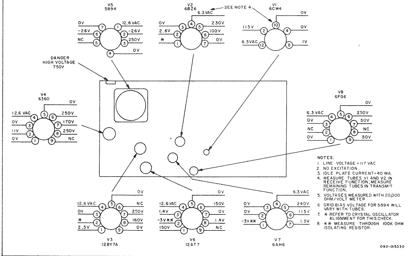
Figure 7. Voltage Chart.
