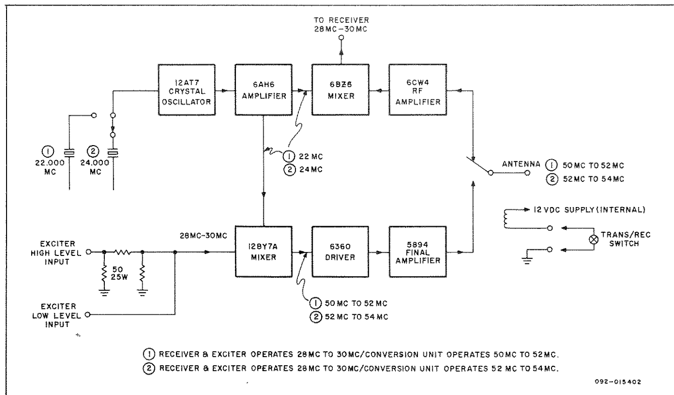
Figure 6. Block Diagram of Transverter.
