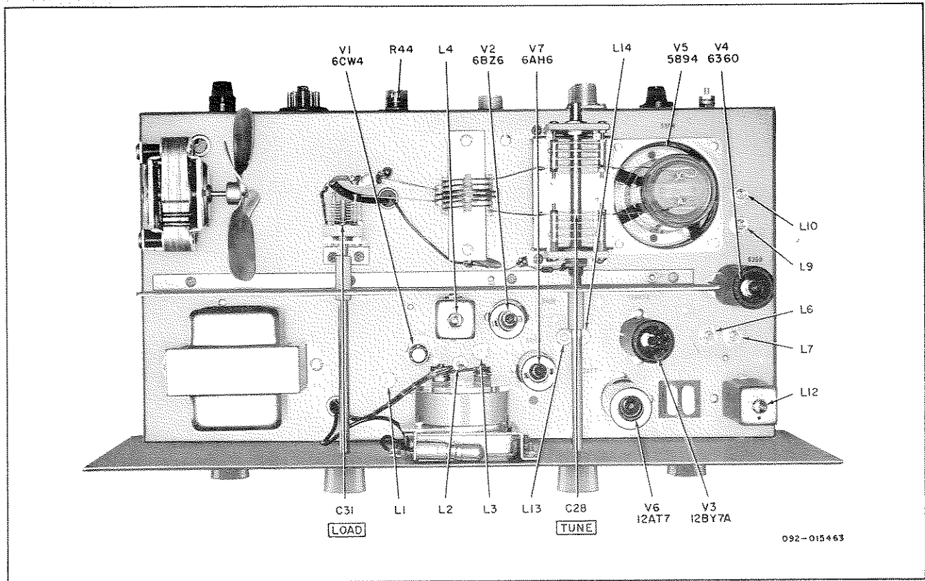
Figure 9. Top View of Transverter Chassis.
