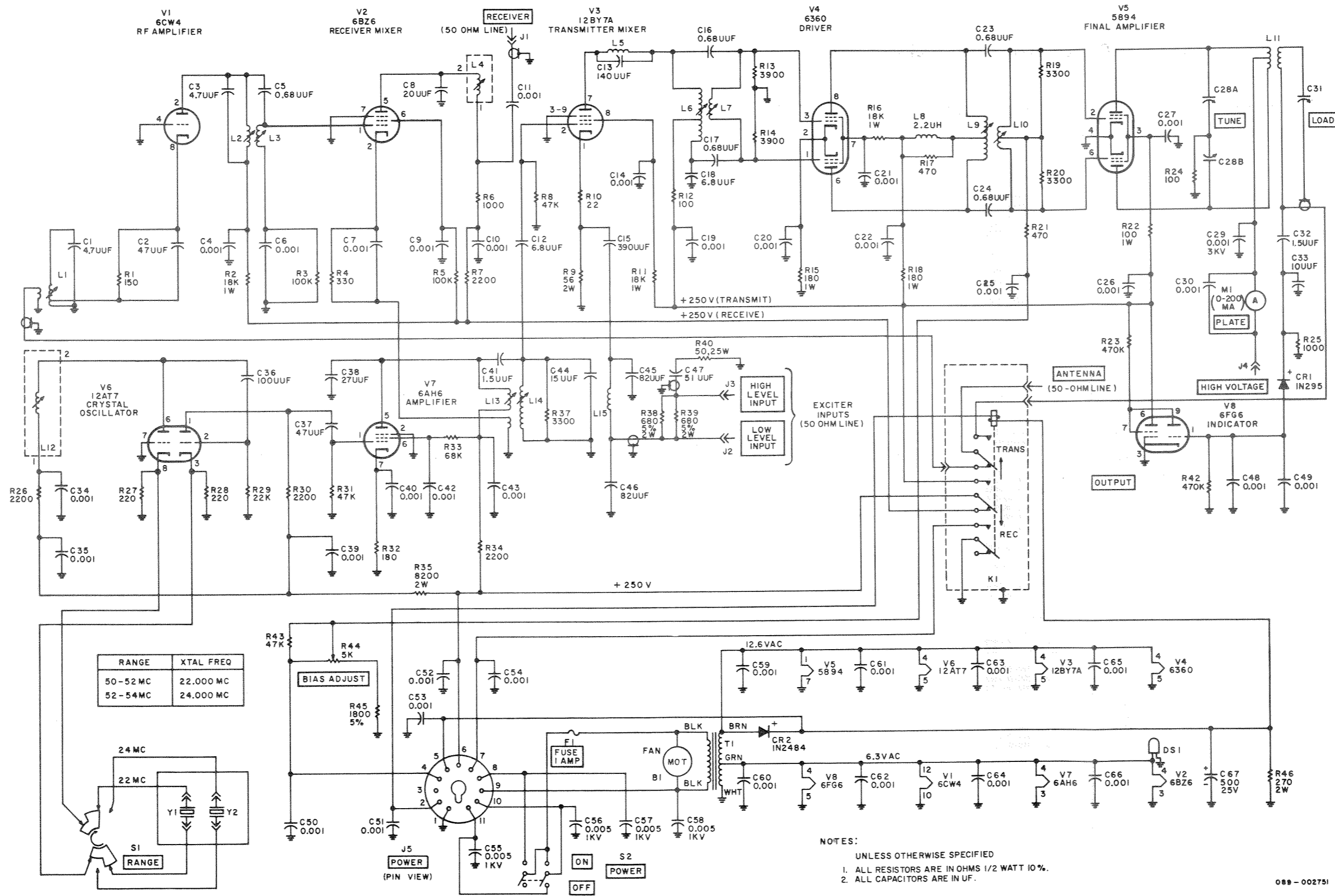
Figure 16. Schematic Diagram of the Model HA-6 Six-Meter Transverter.
