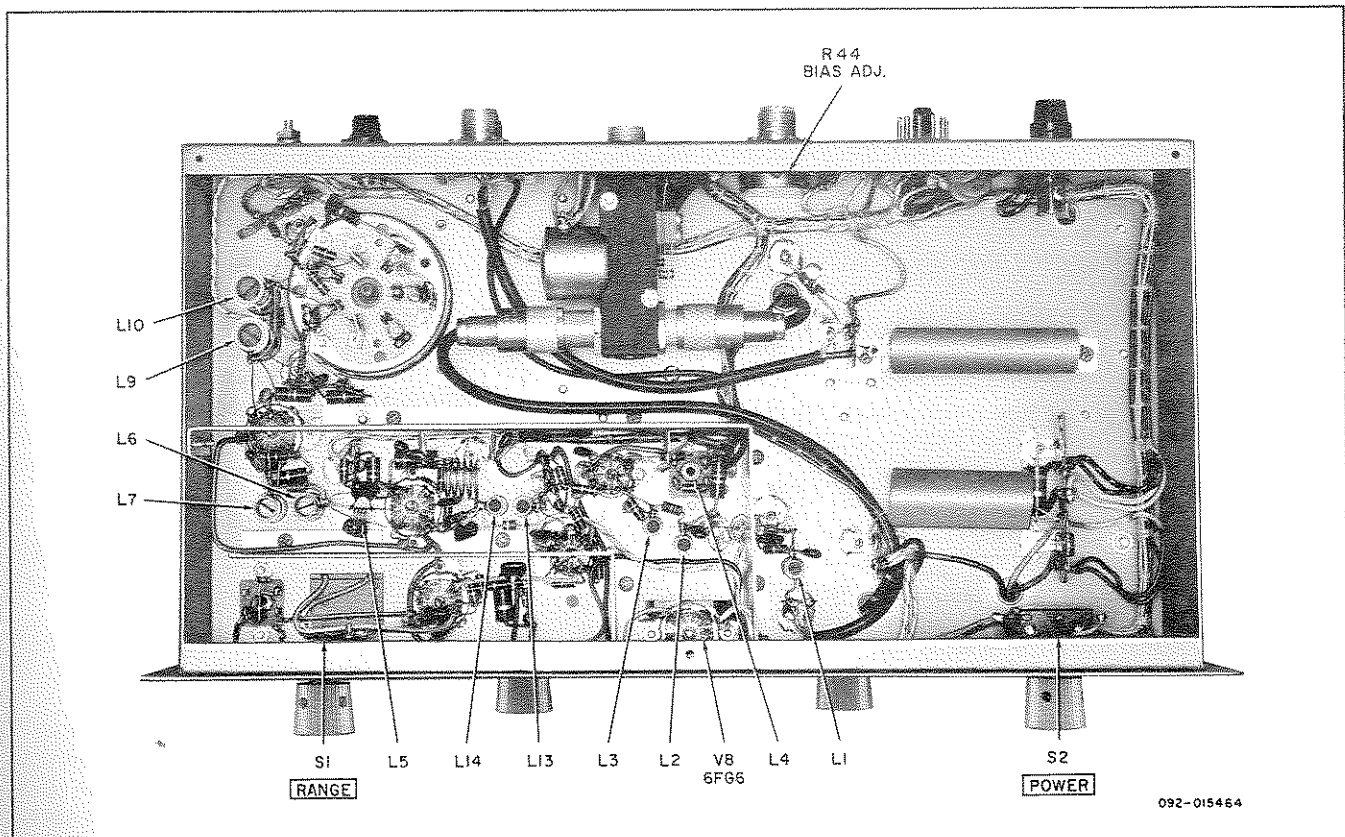
Figure 10. Bottom View of Transverter Chassis.
