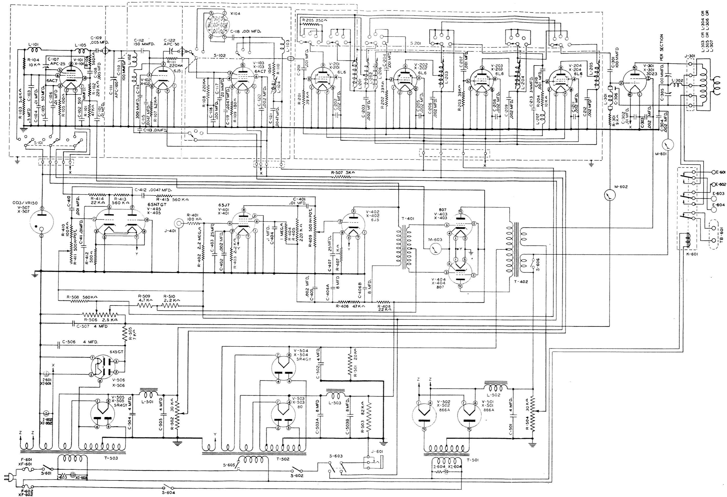
FIG. #1 SCHEMATIC DIAGRAM
