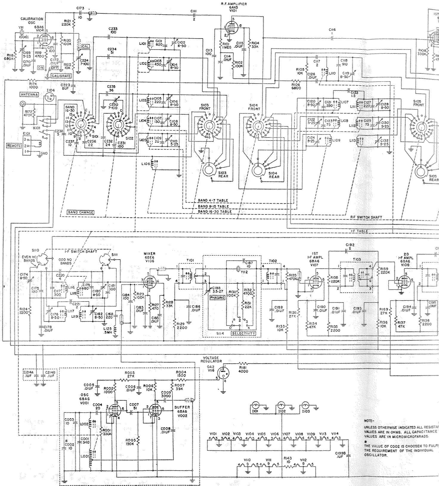
Figure 42. Radio receiver R-388/URR.
