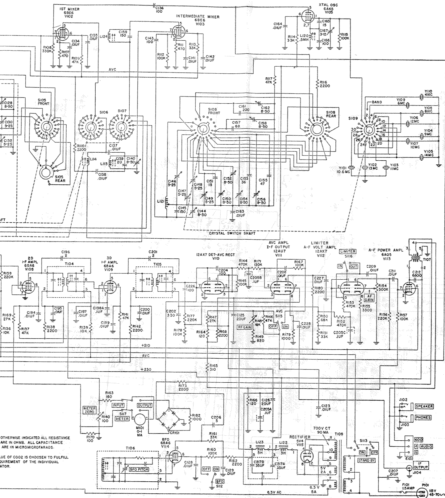
Receiver R-388/URR, over-all schematic.
